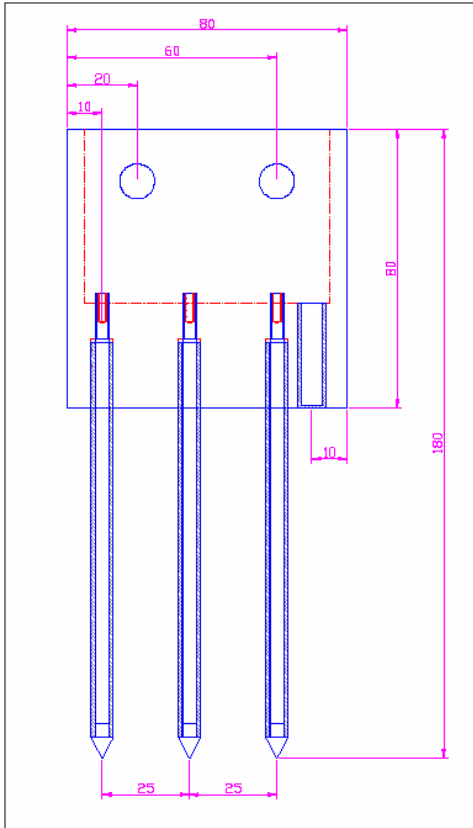
WS3 probe head mechanical dimensions
